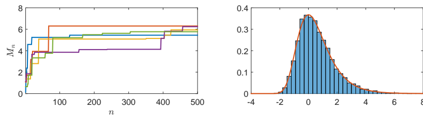
(a) Illustrations of five sample paths of extremal process (b) Histogram of M_n - \log(n) for n = 500 over 5000 realizations. The orange line is the density function of \Lambda
