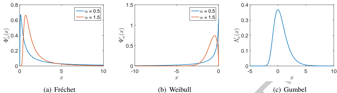
Figure 7.4: Probability density functions corresponding to the standard max-stable distributions
