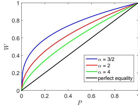
Figure 1.5: Lorenz curves for the Pareto distribution: Lorenz curves for different values of \alpha . Note that the smaller the value of \alpha , the more pronounced the concentration of wealth within a small fraction of the population. The black line represents perfect equality, i.e., the utopian scenario where all individuals have exactly the same wealth.
