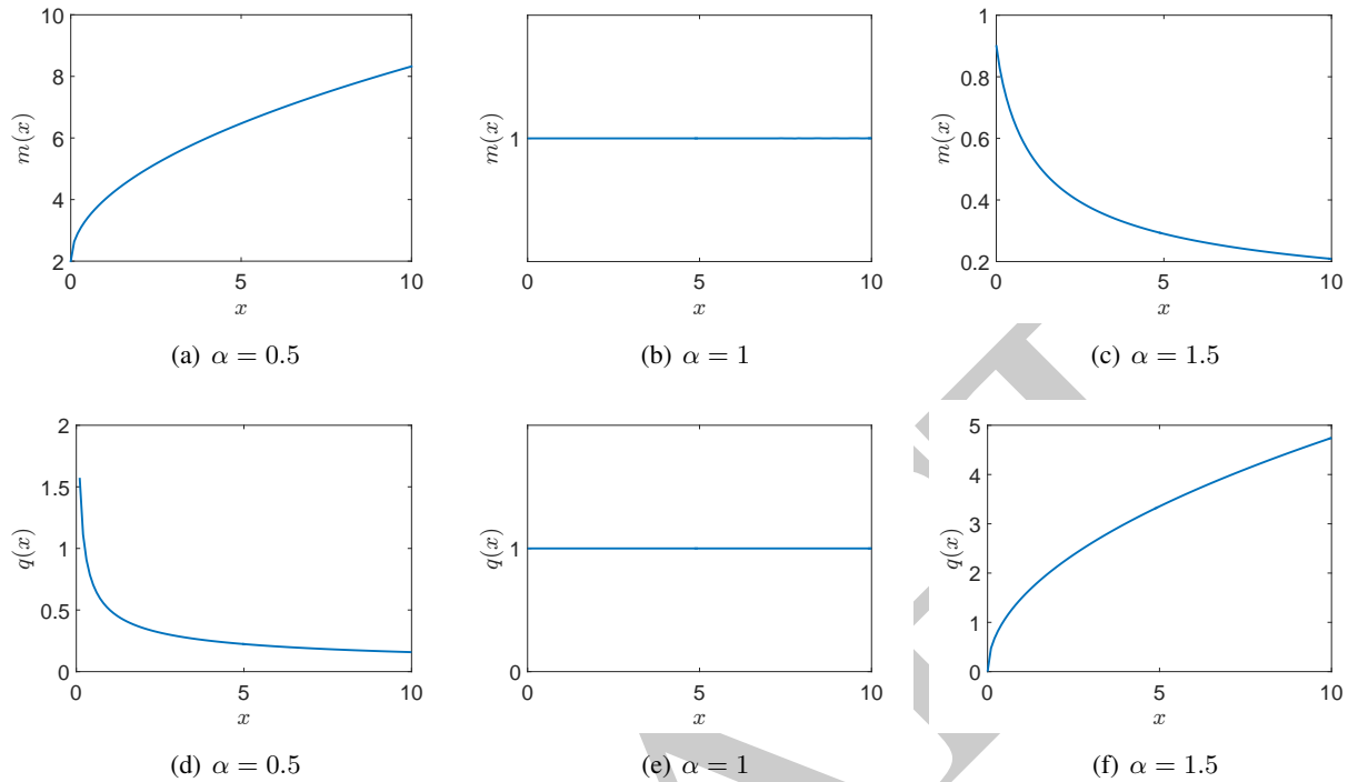
Figure 4.2: Mean residual life and hazard rate of the Weibull distribution with \beta = 1 and different values of \alpha . Recall that \alpha = 1 corresponds to the Exponential distribution.
