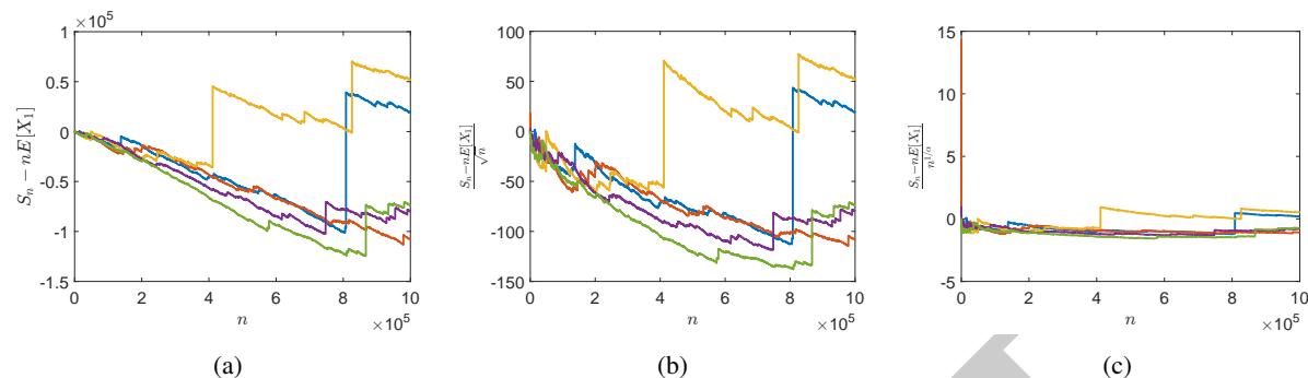
Figure 5.3: Illustration of the error of the first-order approximation of S_n provided by the law of large numbers for Pareto distributed X_1 with \alpha = 1.2 and mean 1 (note that X_1 has an infinite variance). The plots illustrate 5 realizations of S_n - n\mathbb{E}[X_1] , each showing a different scaling: (a) shows the unscaled deviation around the mean; (b) shows the classical central limit theorem scaling, which does not lead to a limiting distribution; and (c) shows the generalized central limit theorem scaling, which leads to a non-Gaussian limiting distribution.
