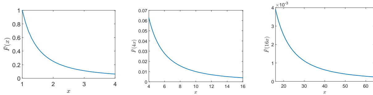
Figure 2.2: The c.c.d.f. corresponding to the Pareto distribution ( \alpha = 2 , x_m = 1 ) plotted at different scales of the independent variable. Note that the shape of the curve is preserved up to a multiplicative scaling, consistent with scale invariance.
