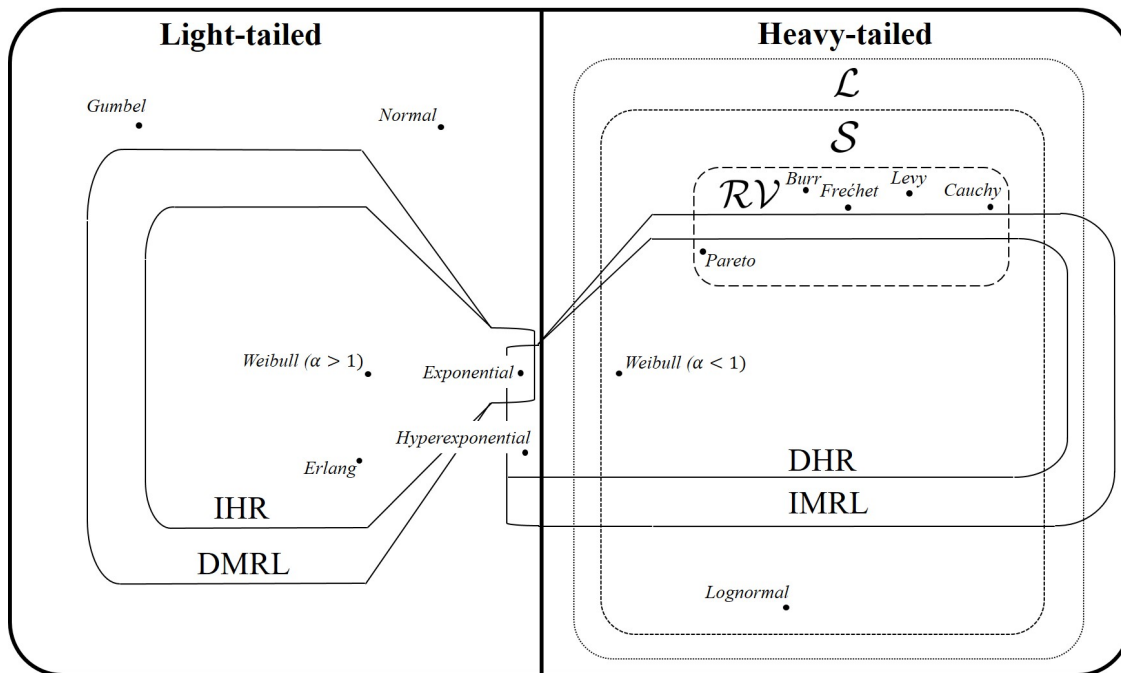
Figure 4.4: Illustration of various classes of heavy-tailed distributions, along with common distributions.
