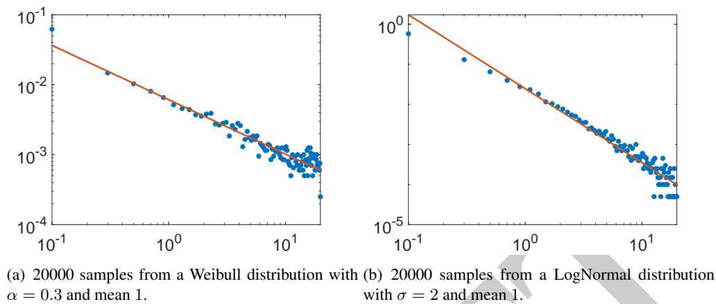
Figure 8.8: Histograms corresponding to samples from a heavy-tailed Weibull (Fig (a)) and a LogNormal (Fig (b)) distribution. The least squares regression line has an R^2 of 0.92 in the case of the Weibull, and 0.94 in the case of the LogNormal
