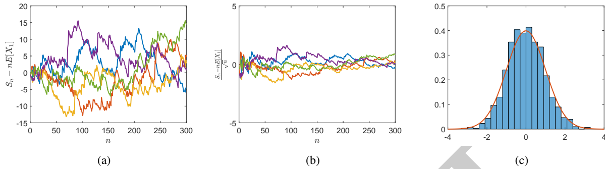
Figure 5.2: Illustration of the second-order approximation of S_n provided by the central limit theorem. The plots illustrate 5 realizations of S_n with X_i \sim \text{Exp}(1) for n = 300 . (a) shows the error of the first-order approximation provided by the law of large numbers, i.e., S_n - n\mathbb{E}[X_i] . (b) shows the normalized error of the first-order approximation, i.e., (S_n - n\mathbb{E}[X_i])/\sqrt{n} . (c) shows the histogram of the normalized error of the first-order approximation for n = 300 over 1000 sample paths. The red curve is the probability density function of the standard Gaussian distribution.
