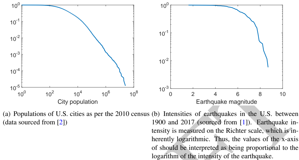
Figure 2.4: Empirical c.c.d.f. (a.k.a. rank plot) corresponding to two real world datasets on a log-log scale.
