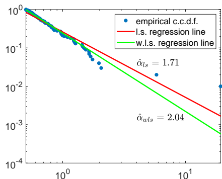
Figure 8.9: Rank plot corresponding to 100 samples from a Pareto distribution with x_m = 0.5 and \alpha = 2 , alongside the least squares and weighted least squares regression lines. Note that the least-squares regression line is ‘swayed’ by the considerable tail noise in the rank plot. Clearly, the weighted least squares estimate of the tail index is more accurate.
