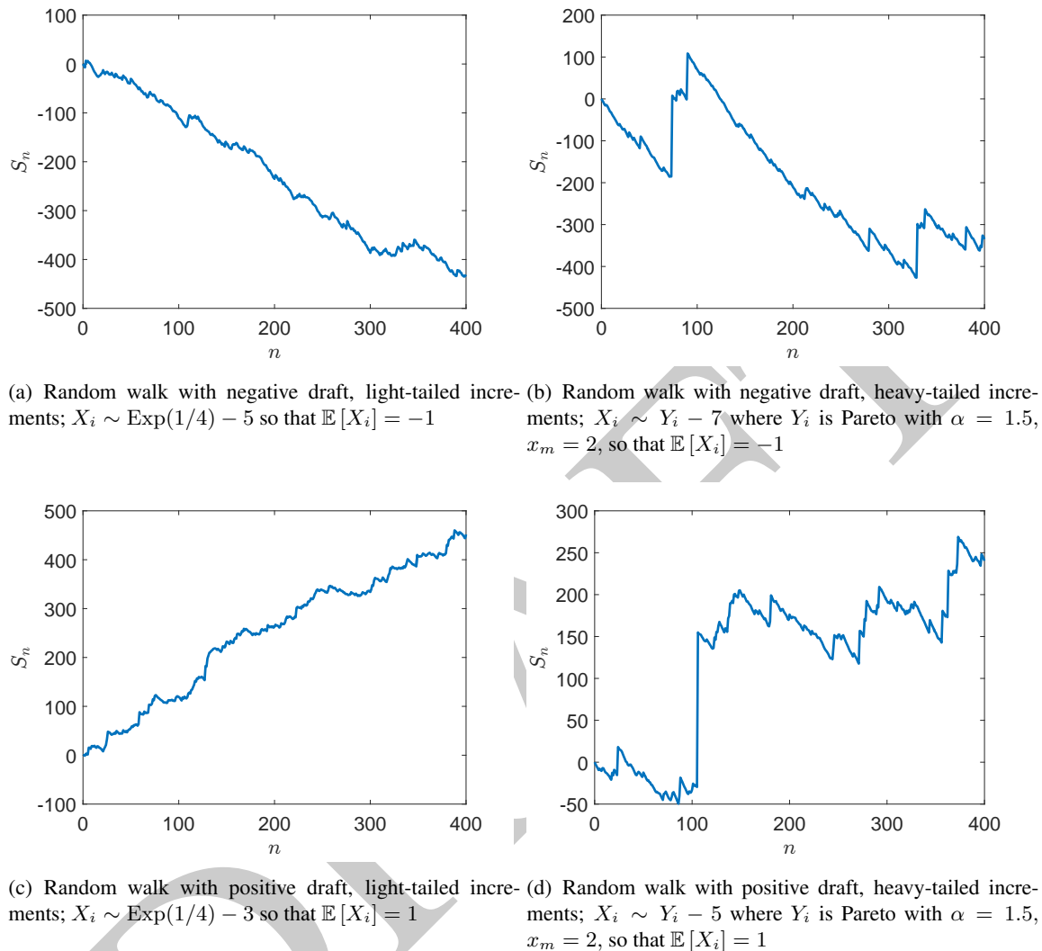
Figure 7.8: Illustrations contrasting the behavior of random walks with negative/positive drifts and light-tailed/heavy-tailed increments.
