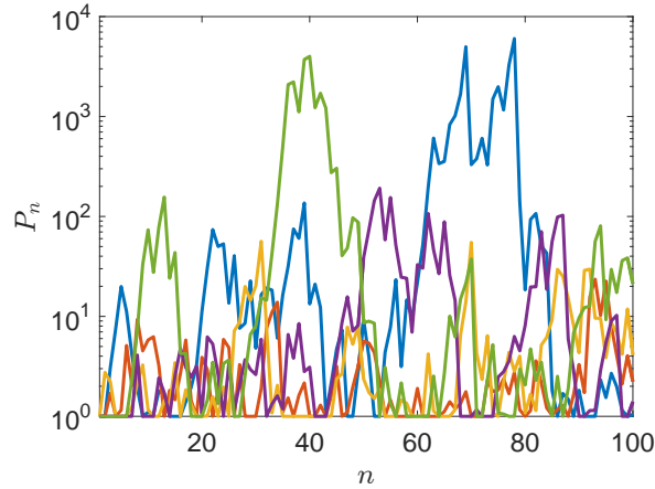
Figure 6.2: Illustration of a multiplicative process with a lower barrier. The plots show 5 realizations of P_n with Y_i \sim \text{Exp}(3/4) and l = 1 . Note that the process gets occasionally ‘reset’ to the lower barrier, but can take large values between successive resets.
