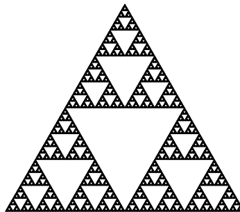
Figure 2.1: Illustration of the Sierpinski fractal [135].
