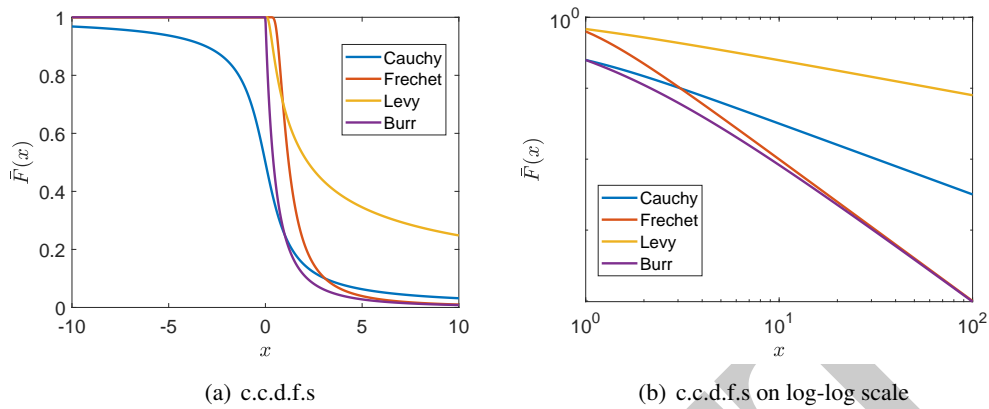
Figure 1.9: The plots show the c.c.d.f. of the standard Cauchy ( x_0 = 0, \gamma = 1 ), the Fréchet (with x_m = 0, \beta = 1, \alpha = 2 ), the Lévy (with \mu = 0, c = 1 ), and the Burr distribution (with c = \lambda = 1, k = 2 ). Fig. (a) shows the plots on a linear scale, and Fig. (b) on a log-log scale. Note that all c.c.d.f.s look (asymptotically) linear on a log-log scale; we will formalize this property in Chapter 2.
