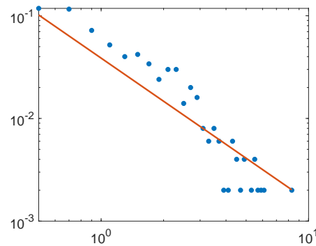
Figure 8.4: Histogram of 500 samples from an Exponential distribution ( \mu = 1 ) plotted on a log-log scale, along with the best fit regression line.
