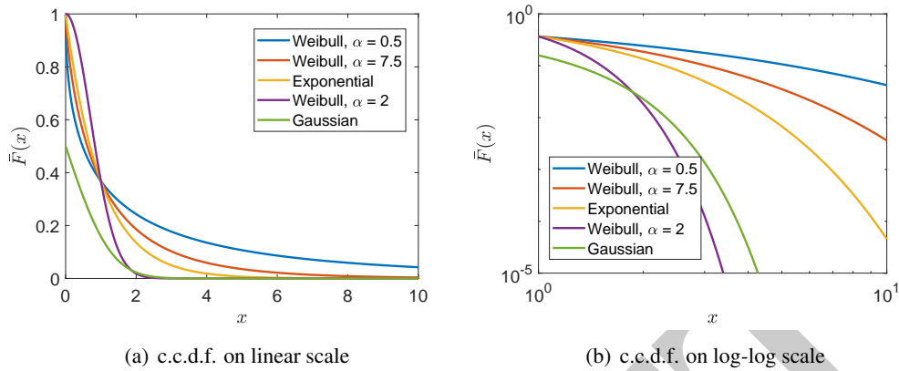
Figure 1.6: Illustration of Weibull c.c.d.f.: Plots show the c.c.d.f. of the Weibull distribution with scale parameter \beta = 1 and different values of shape parameter \alpha , alongside the Exponential distribution (with unit mean, which corresponds to \alpha = \beta = 1 ) and the standard Gaussian. Fig. (a) shows the c.c.d.f.s on a linear scale, while Fig. (b) plots them on a log-log scale.
