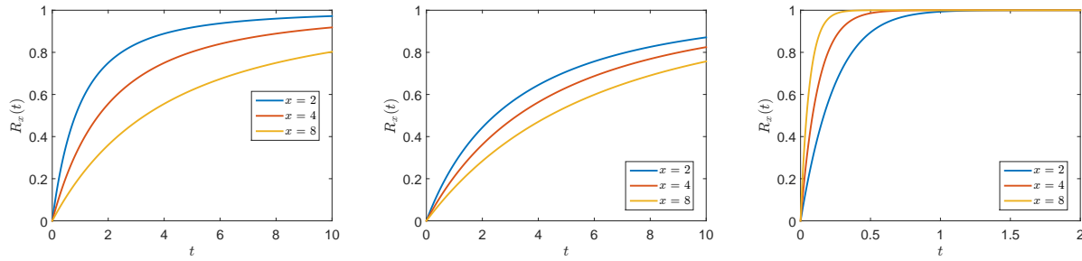
(a) Pareto distribution: x_0 = 1, \alpha = 2 (b) heavy-tailed Weibull: \beta = 1, \alpha = 1/2 (c) light-tailed Weibull: \beta = 1, \alpha = 2
