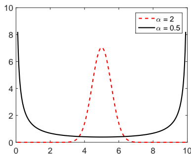
Figure 3.1: A visualization of the conspiracy and catastrophe principles under the Weibull distribution. The conditional density function of X_1 given that X_1 + X_2 = 10 is shown, where X_1 and X_2 are i.i.d. Weibull random variables that are either light-tailed ( \alpha = 2 ) or heavy-tailed ( \alpha = 0.5 ).
