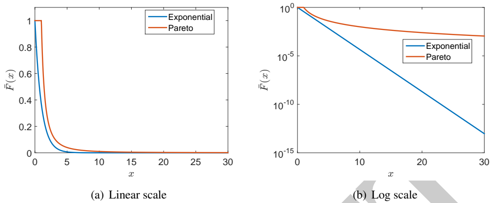
Figure 1.1: Contrasting heavy-tailed and light-tailed distributions: The plots show the c.c.d.f. of the exponential distribution (with mean 1) and a heavy-tailed Pareto distribution (with x_m = 1 , scale parameter \alpha = 2 ). While the contrast in tail behavior is difficult to discern on a linear scale (Fig (a)), it is quite evident when the probabilities are plotted on a logarithmic scale (Fig (b)).
