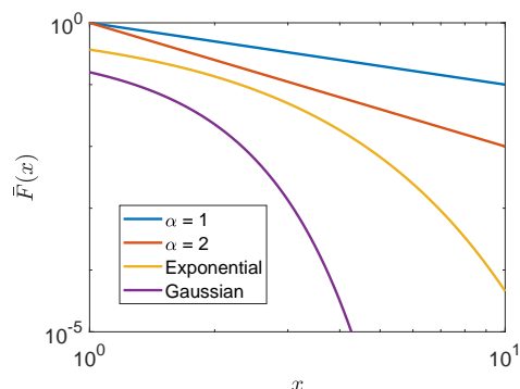
Figure 1.3: A clearer contrast between the Pareto distribution and the Exponential/Gaussian: The plots show the c.c.d.f. corresponding to different Pareto distributions with x_m = 1 with different values of \alpha , alongside the Exponential distribution (with unit mean) and the standard Gaussian, on a log-log scale. Notice how this scaling demonstrates clearly how the Pareto tail (linear on a log-log plot) is heavier than that of the Exponential and the Gaussian.
