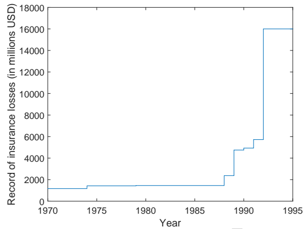
Figure 7.2: Record of insurance loss due to catastrophies worldwide in millions of US Dollars (at 1992 prices) between 1970–1995 [163].
