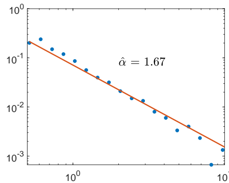
Figure 8.5: Histogram of 3000 samples from a Pareto distribution with x_m = 0.5 \alpha = 2 , using logarithmic binning; each bin has width 10 times the width of the previous one, to create 40 bins over the interval [0.1, 10] . Bin centers are chosen to be the geometric means of the bin boundaries.
