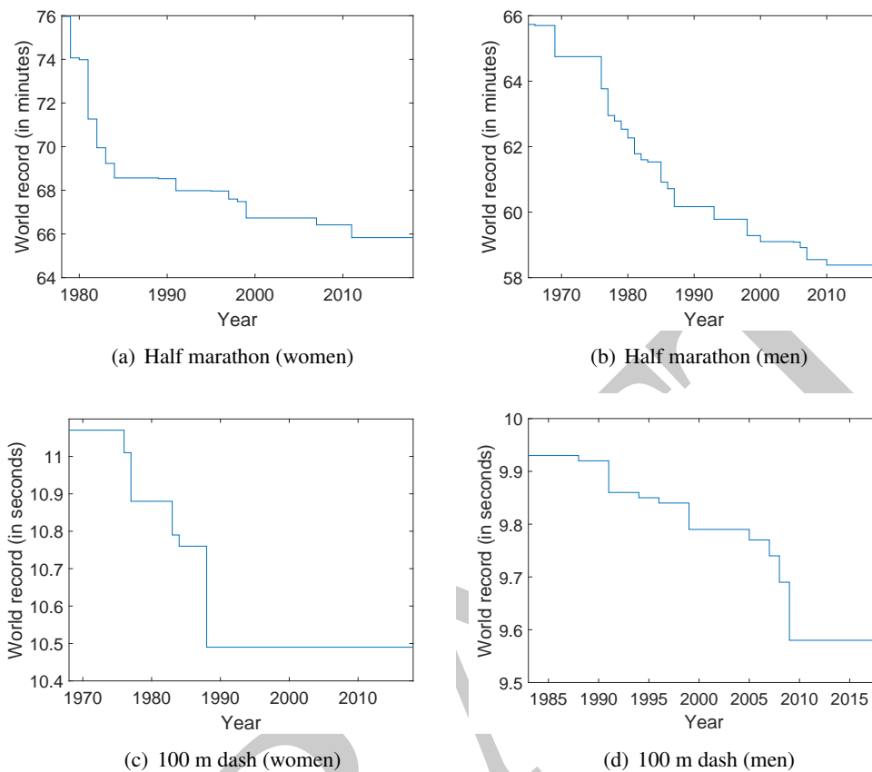
Figure 7.1: Progression of world record as ratified by the International Association of Athletics Federations (IAAF).
