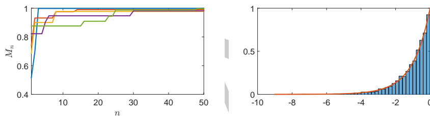
(a) Illustrations of five sample paths of extremal process (b) Histogram of n(M_n - 1) for n = 50 over 5000 realizations. The orange line is the density function of \Psi_1
