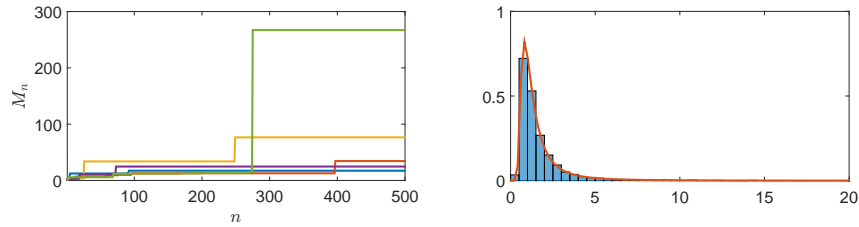
(a) Illustrations of five sample paths of extremal process (b) Histogram of \frac{M_n}{\sqrt{n}} for n = 500 over 5000 realizations. The orange line is the density function of \Phi_2 .
