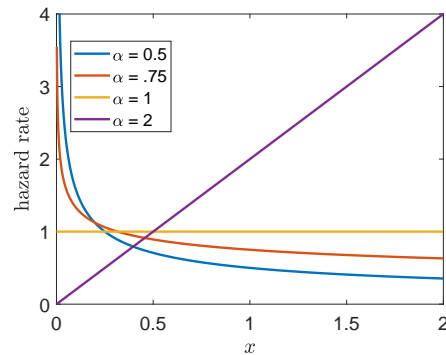
Figure 1.7: Weibull hazard rate for scale parameter \beta = 1 and different values of shape parameter \alpha
