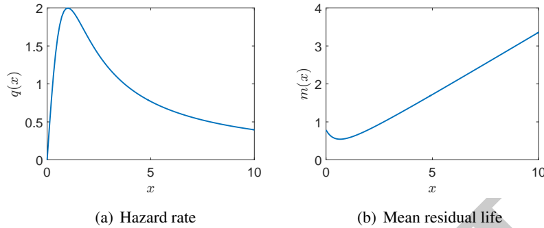
Figure 4.3: Hazard rate and mean residual life for the Burr distribution, with \lambda = 1 , c = k = 2 . Note that the distribution, though heavy-tailed, is neither IMRL nor DHR.
