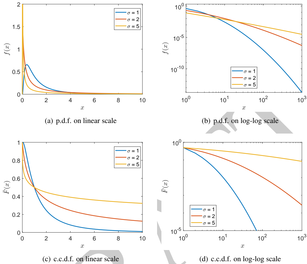
Figure 1.8: Illustration of LogNormal distribution: The c.c.d.f. and p.d.f. of LogNormal distributions with \mu = 0 and different values of \sigma are depicted. The p.d.f.s are plotted on a linear scale in Fig. (a), and on a log-log scale in Fig. (b). The corresponding c.c.d.f.s are plotted on a linear scale in Fig. (c), and on a log-log scale in Fig. (d). Note that the p.d.f. as well as the c.c.d.f. appears nearly linear on a log-log plot when \sigma is large.
