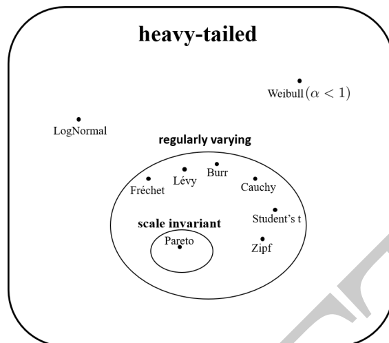
Figure 2.5: Scale invariant and regularly varying distributions.
