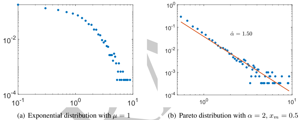
Figure 8.3: Histograms on a log-log scale
