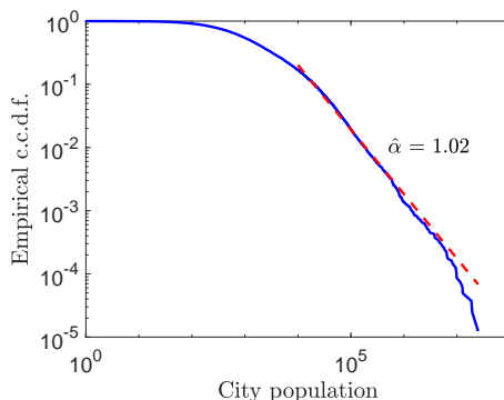
Figure 1.4: Visualizing data on a log-log plot: The figure shows the empirical c.c.d.f. of the populations of U.S. cities as per the 2010 census (data sourced from [2]). Note that on a log-log scale, the data beyond population 10^4 looks approximately linear. The least squares regression line on this data yields a estimate \hat{\alpha} = 1.02 of the power law exponent.
