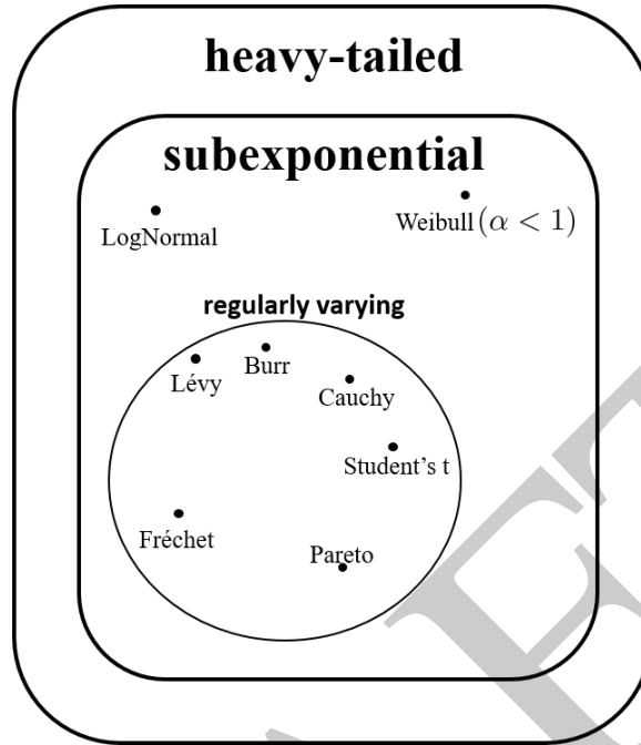
Figure 3.2: Illustration of the relationship of the class of subexponential distributions to other heavy-tailed distributions.
