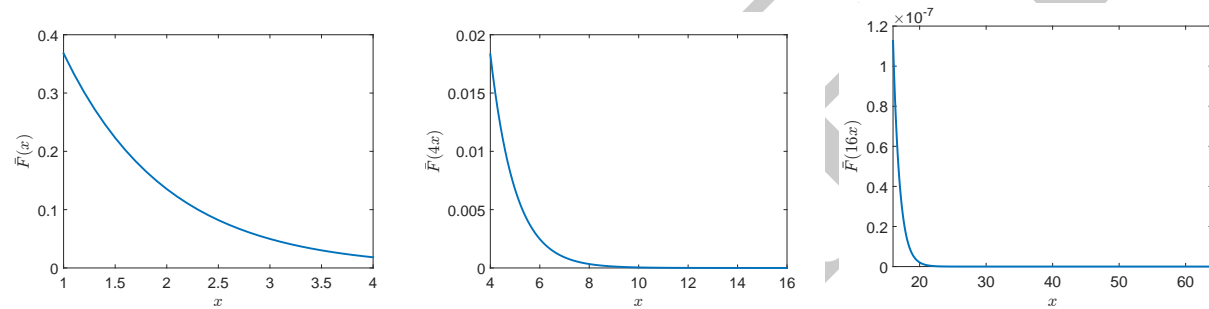
Figure 2.3: The c.c.d.f. corresponding to the Exponential distribution (with mean 1) plotted at different scales of the independent variable. Note that the shape of the curve looks fundamentally altered at different scales.
