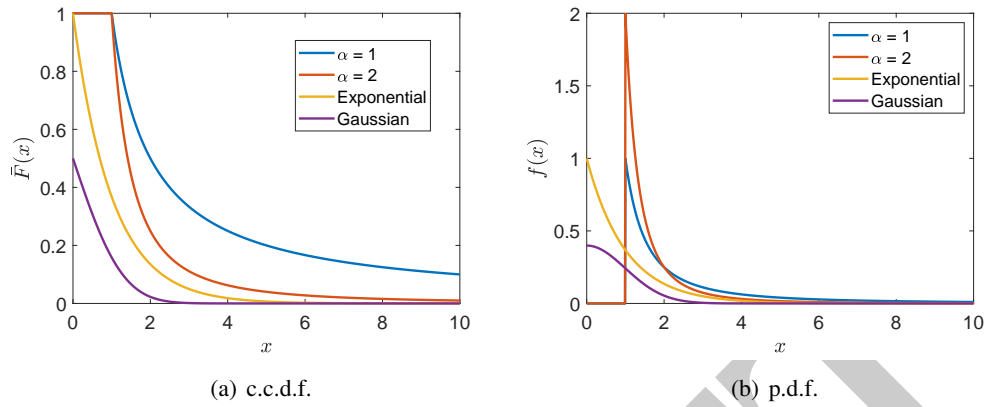
Figure 1.2: Contrasting Pareto distribution with the Exponential and the Gaussian: The plots show the c.c.d.f. (Fig. (a)) and p.d.f. (Fig. (b)) corresponding to different Pareto distributions with x_m = 1 with different values of \alpha , alongside the Exponential distribution (with unit mean) and the standard Gaussian.
