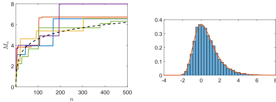
Figure 7.3: Illustration of an extremal process. (a) shows five realizations of M_n with X_i \sim \text{Exp}(1) . The dotted line is the first order approximation \log(n) . (b) shows a histogram of the error M_n - \log(n) of the first first order approximation for n = 500 over 5000 realizations. The orange curve is the probability distribution function of the Gumbel distribution.
