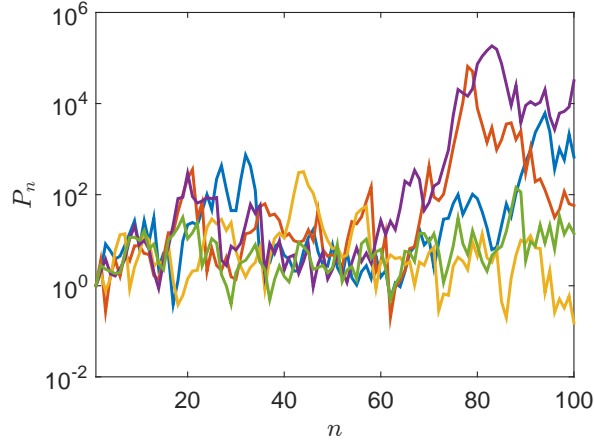
Figure 6.3: Illustration of a multiplicative process with additive noise. The plots show 5 realizations of P_n with Y_i \sim \text{Exp}(0.75) , Q_i being distributed as the absolute value of a standard Gaussian.
