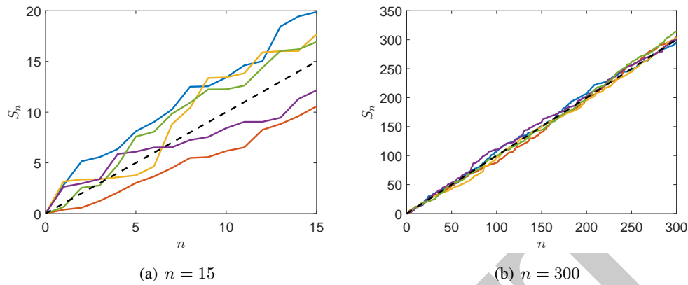
Figure 5.1: Illustration of the first-order approximation of S_n provided by the law of large numbers. The plots illustrate 5 realizations of S_n with X_i \sim \text{Exp}(1) . The dotted line shows the law of large numbers approximation.
