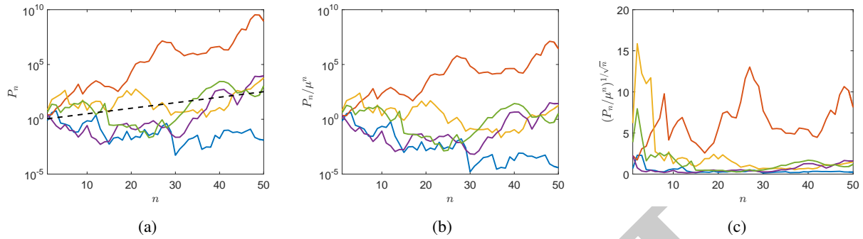
Figure 6.1: Illustration of the multiplicative process P_n . The plots illustrate 5 realizations of P_n with Y_i \sim \text{Exp}(1/2) . Figure (a) shows the (unscaled) process itself. Note that the scale on the y-axis is logarithmic, indicating an exponential growth in the process P_n . The dotted line is the first-order approximation \mu^n , where \mu = e^{\mathbb{E}[\log(Y_1)]} . Figure (b) shows the same process normalized with respect to the first order approximation. Note that the y-axis is still on a logarithmic scale. Finally, Figure (c) shows the process scaled as per the multiplicative central limit theorem. Note that the y-axis is now linear. Under this scaling, Theorem 6.1 shows that the process converges in distribution to the LogNormal distribution.
